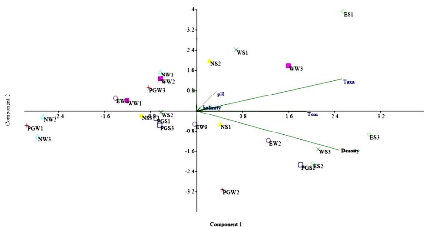
Figure 7: Principle Component Analysis (PCA) to consider the correlation between ballast water parameters and phytoplankton density in the ballast water tanks of entered ships to Shahid Rajaee Port, Hormozgan, Iran.
